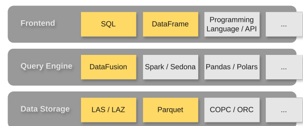
Figure 1. Lakehouse architecture for point cloud data analytics.
