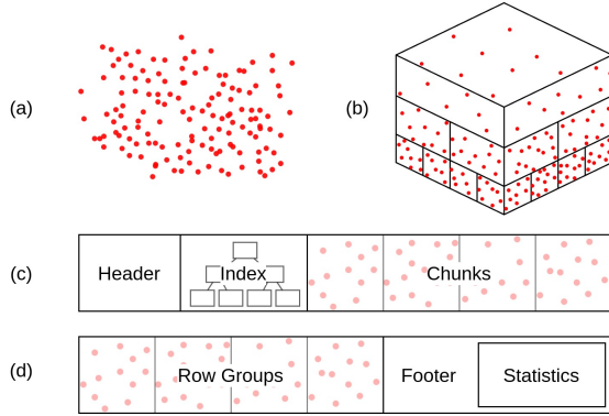
Figure 3. Data organization for point cloud visualization.
