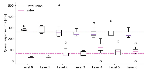
Figure 4. Visualization query performance on different levels.
