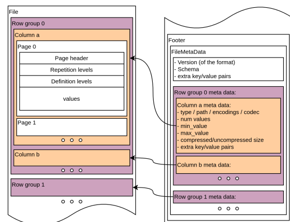
Figure 2. The Apache Parquet file format layout.
