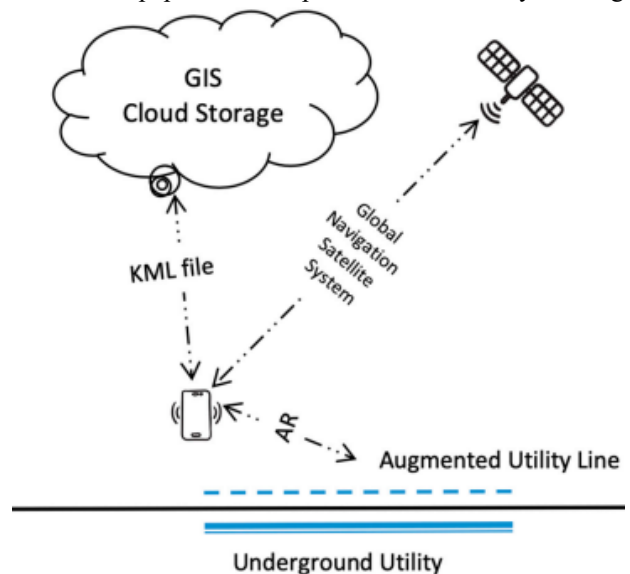
Figure 1. A workflow for the development of AR in combination with GIS. Source: Fenais et al., 2019.
