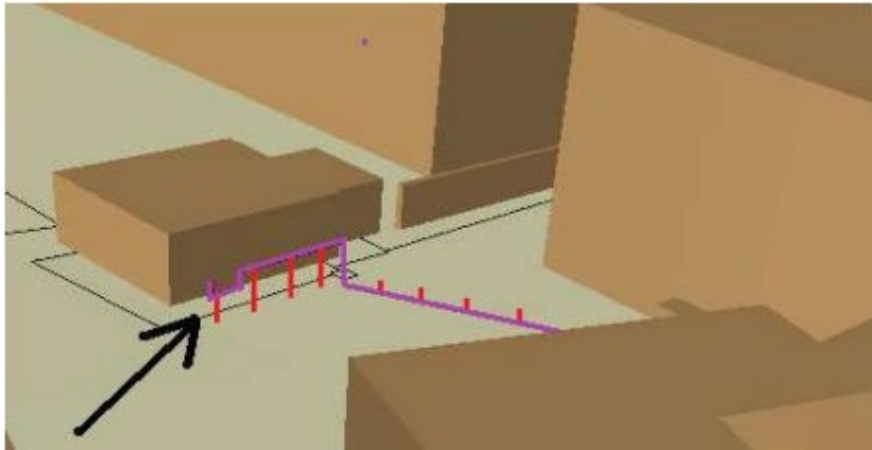
Figure 2. A pipeline that starts above ground and goes partly underground. The black lines on the surface are the normal parcel boundaries, and the vertical reference features show the vertical distance to the surface, indicating whether it is above or below the ground surface and the depth or height. This information can be switched on or off. Source: Vandyshveva et al. 2012. In Van Oosterom, 2018, p 203.
