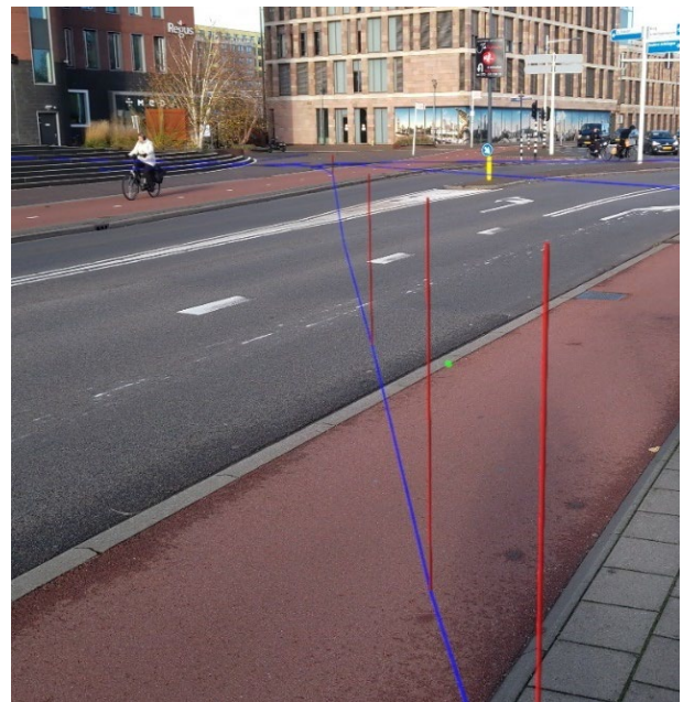
Figure 5. Vertical reference features at a controlled directional drilling location of the water network. The vertical reference features bridge the gap from the depth of the pipe to the ground surface. The vertical reference features give perspective in AR for the precise location of the pipe in relation to the depth.
